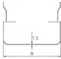
湿帘下框 Pad bottom frame L=6m, w=150mm
