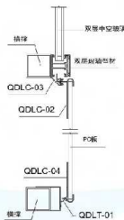
侧窗安装方式 Installation of side window profiles
