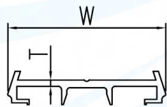
压板 middle plate LCBL-02 L=6000mm, W=47mm, T=1.8mm
