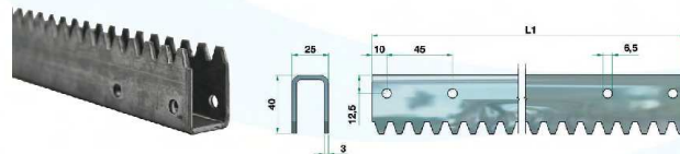
拉幕齿条 Screening rack L1= 2965, 3965 4965 mm T= 2.75mm 3mm
