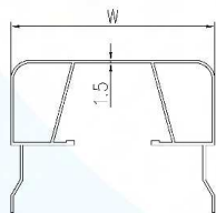
湿帘上框 Pad cover frame
