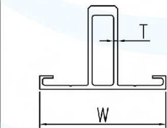
底板 Bottom plate LCBL-04 L=6000mm, W=47mm, T=1.5mm
