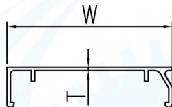
盖板 Pinch plate LCBL-03 L=6000mm, W=59.5mm, T=1mm
