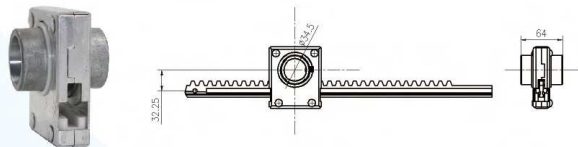
铝合金开窗齿轮 Aluminum ventilation pinion A型, 1" A Type, 1"
